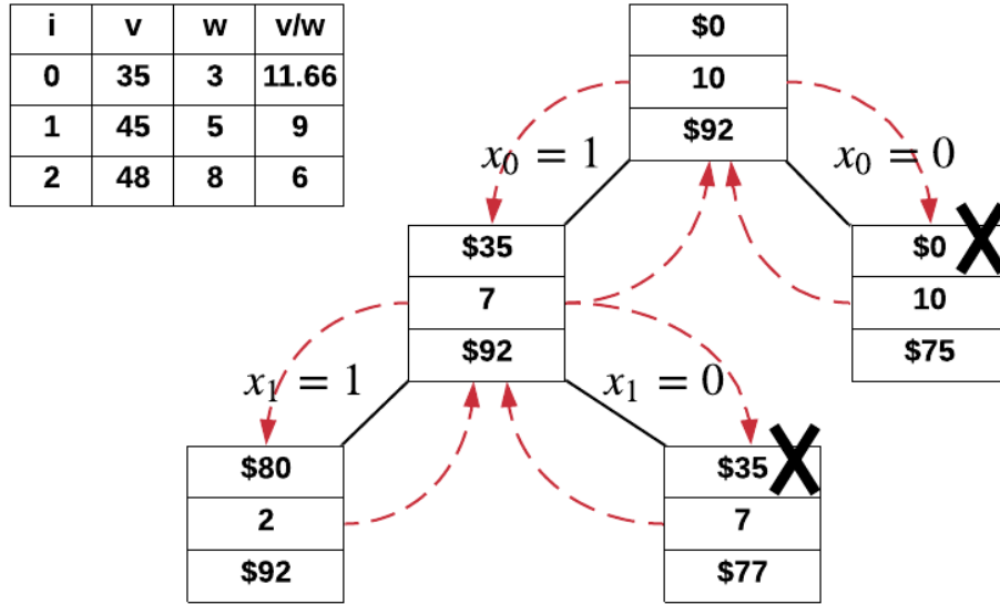
Figure 12.9: Depth-First Branch and bound
