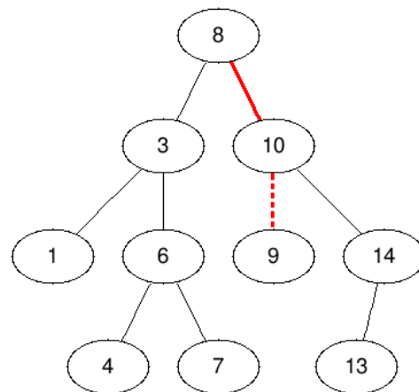
Figure 14.6: The red colored path from the root down to the position where the key 9 is inserted. The dashed line indicates the link in the tree that is added to insert the item.
