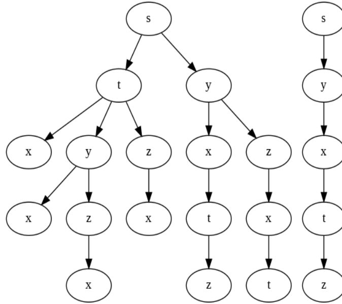
Figure 20.13: All paths from source vertex s for graph in Fig. 20.12 and its shortest paths.
