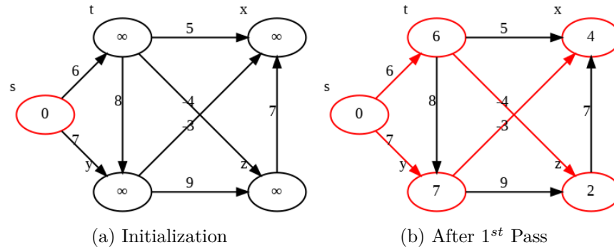
Figure 20.21: The execution of Bellman-Ford's Algorithm on DAG using topologically sorted vertices. The red color marks the shortest-paths tree.
