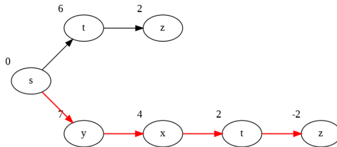
Figure 20.19: The tree structure indicates the updates on D , and the shortest path tree marked by red arrows.
