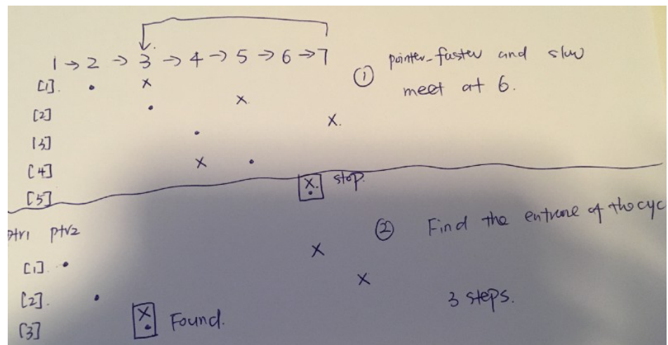
Figure 23.1: Example of floyd's cycle finding
