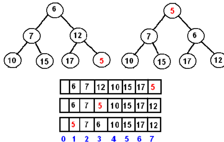
Figure 9.5: A Min-heap.
