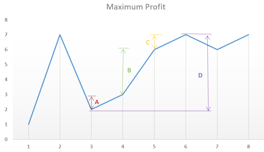
Figure 25.4: profit graph
