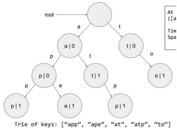
Figure 22.9: Trie Structure
