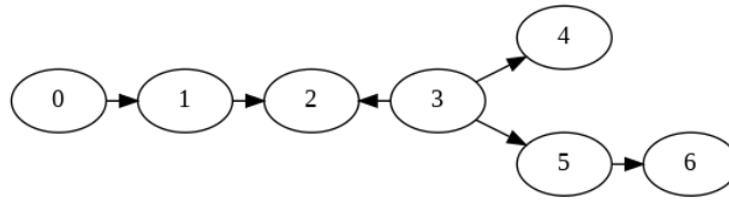
Figure 20.3: DAG 1
