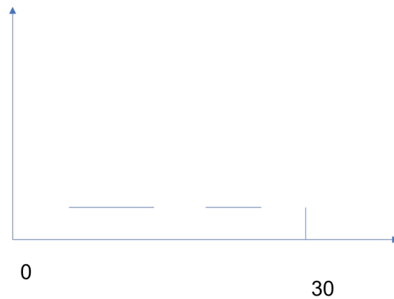
Figure 24.2: Interval questions
