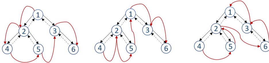
Figure 11.14: Left: PreOrder, Middle: InOrder, Right: PostOrder. The red arrows marks the traversal ordering of nodes.
