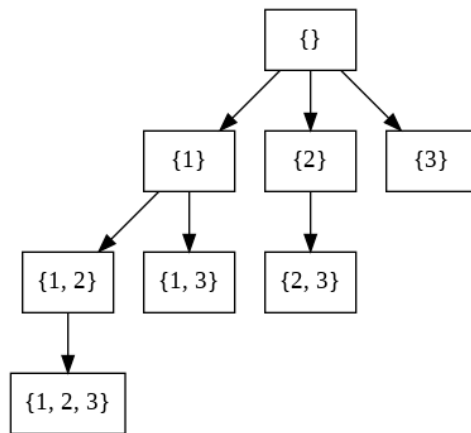
Figure 12.5: The Search Tree of Combination.
