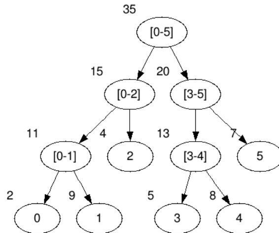
Figure 14.10: Illustration of Segment Tree for Sum Range Query.
