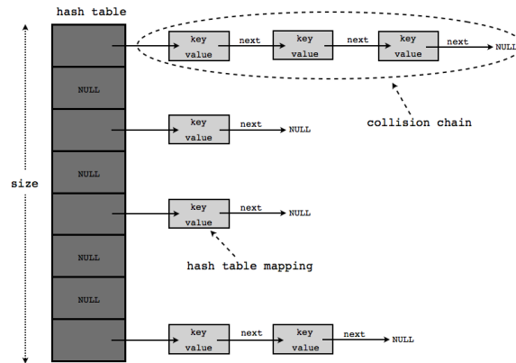
Figure 4.6: Hashtable chaining to resolve the collision, change it to the real example
