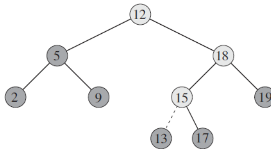
Figure 27.2: The lightly shaded nodes indicate the simple path from the root down to the position where the item is inserted. The dashed line indicates the link in the tree that is added to insert the item.
