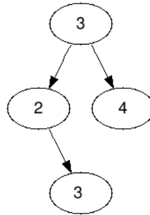
Figure 14.7: A BST with nodes 3 duplicated twice.
