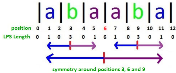
Figure 26.1: LPS length at each position for palindrome.
