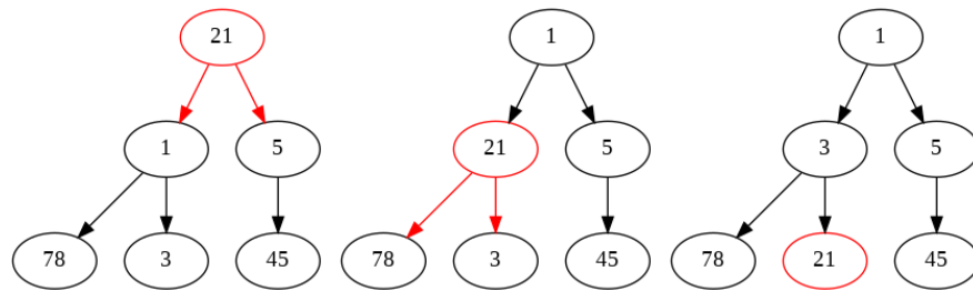
Figure 9.9: Heapify: On node 21.
