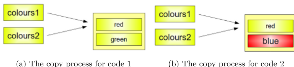
Figure 30.1: Copy process
