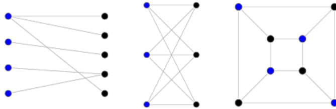
Figure 4.8: Bipartite Graph
