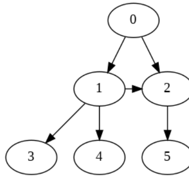
Figure 12.6: Acyclic graph
