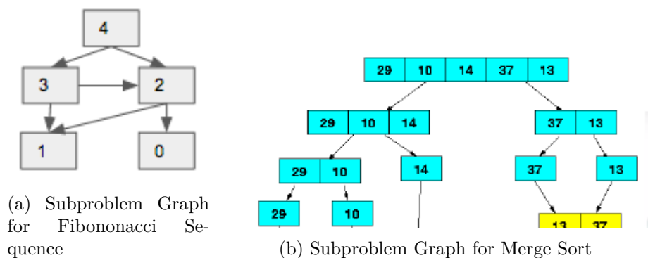
Figure 16.2: Subproblem Graph
