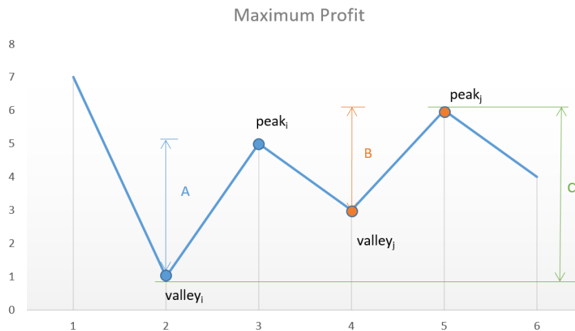
Figure 25.3: Track the peaks and valleys
