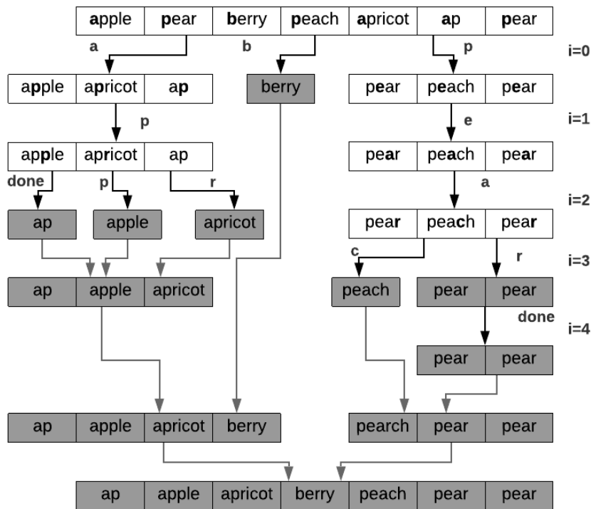
Figure 15.10: Radix Sort: MSD sorting strings in recursion. The black and grey arrows indicate the forward and backward pass in recursion, respectively.
