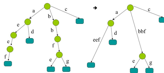
Figure 22.8: Trie VS Compact Trie
