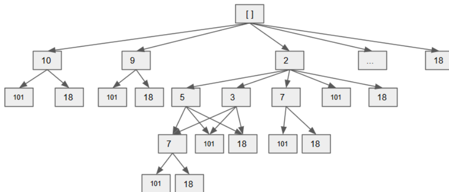
Figure 29.1: State Transfer Tree Structure for LIS, each path represents a possible solution. Each arrow represents an move: find an element in the following elements that's larger than the current node.
