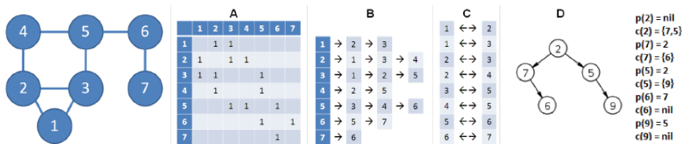
Figure 9.3: Four ways of graph representation, renumerate it from 0. Redraw the graph
