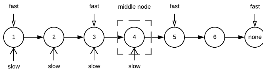
Figure 19.4: Slow-fast pointer to find middle
