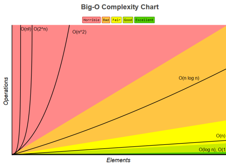
Figure 10.1: Order of Growth of Common Functions
