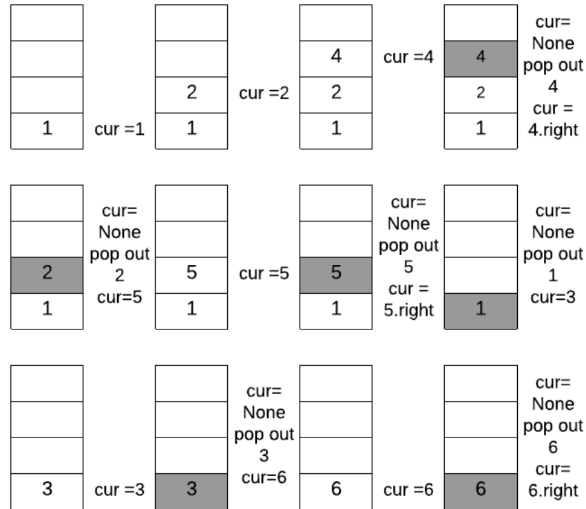
Figure 11.17: The process of iterative tree traversal.
