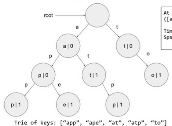
Figure 27.5: Trie Structure
