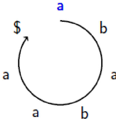
Figure 22.6: Cyclic Shifts
