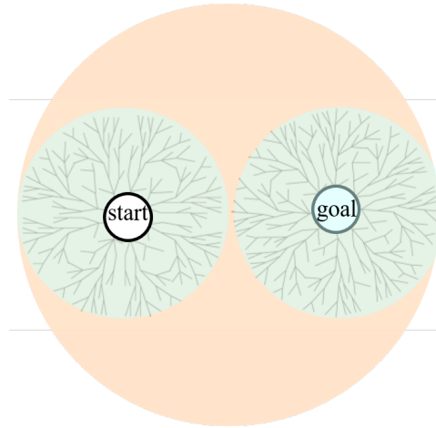
Figure 11.5: Bidirectional search.
