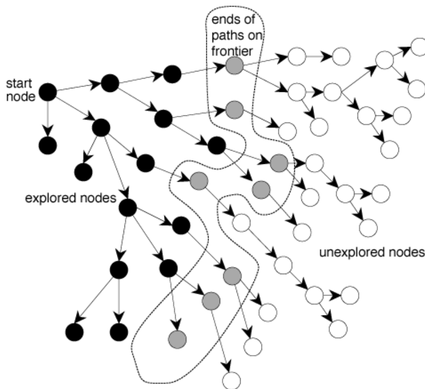
Figure 11.1: Graph Searching
