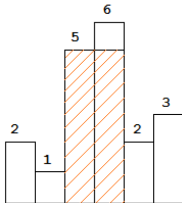
Figure 25.2: Histogram
