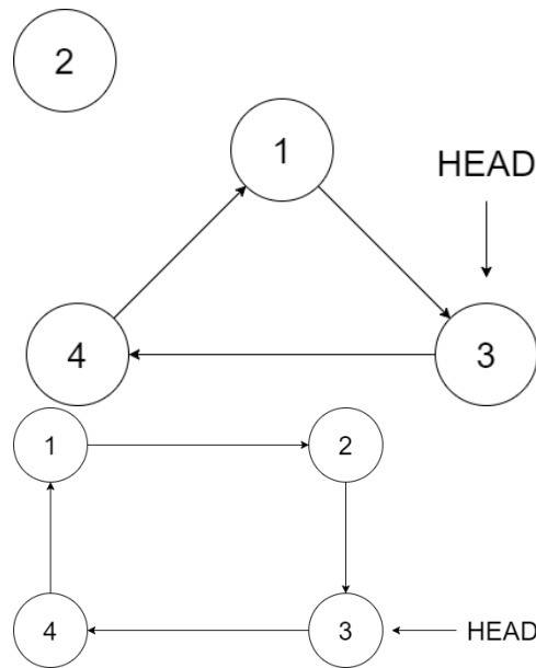
Figure 25.1: Example of insertion in circular list
