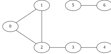
Figure 20.1: Undirected Cyclic Graph. (0, 1, 2, 0) is a cycle
