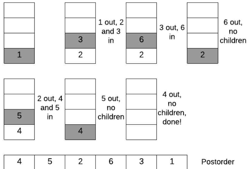
Figure 11.16: The process of iterative postorder tree traversal.
