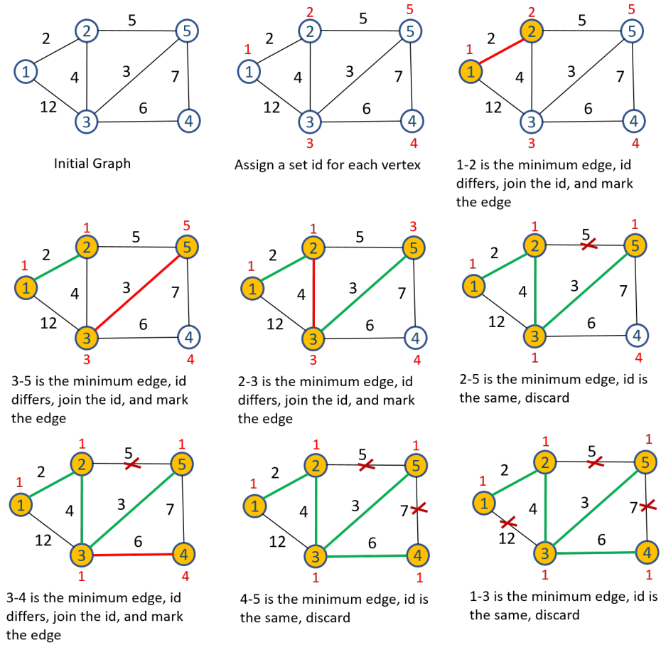
Figure 20.8: The process of Kruskal's Algorithm
