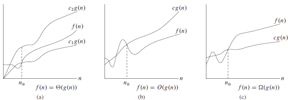
Figure 10.2: Graphical examples for asymptotic notations. Replace f(n) with T(n)
