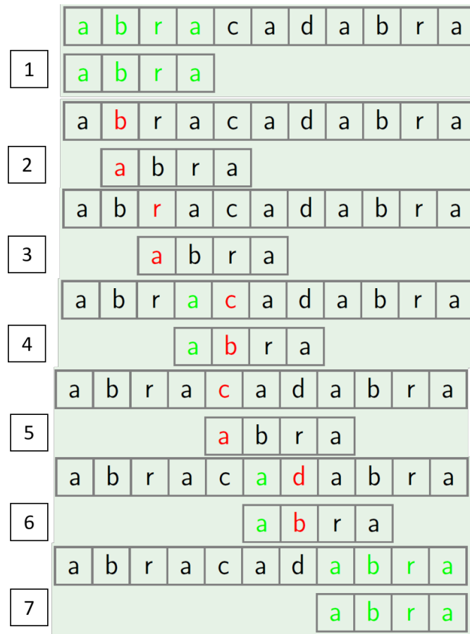
Figure 22.1: The process of the brute force exact pattern matching
