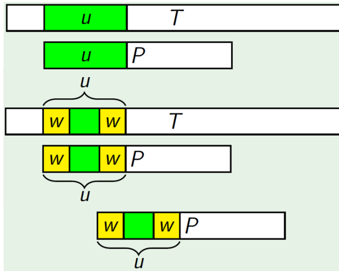
Figure 22.3: The Sliding Rule
