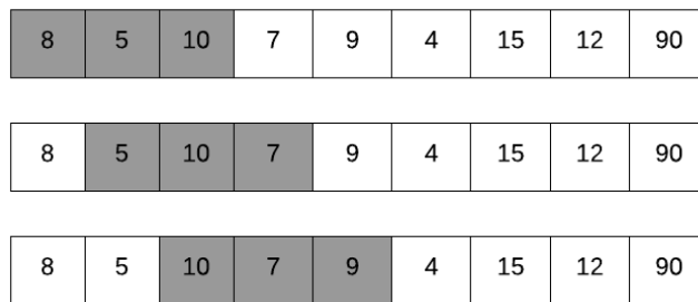
Figure 19.7: Sliding Window Property
