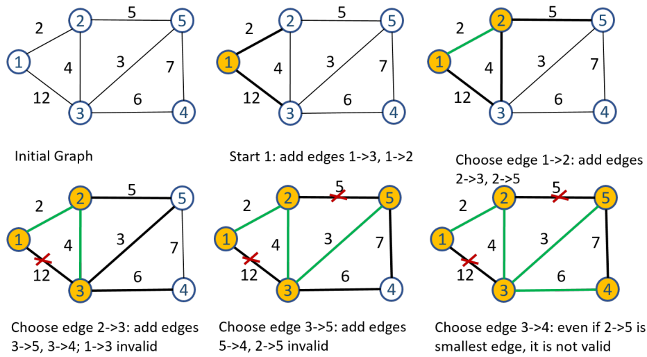
Figure 20.10: Prim's Algorithm, at each step, we manage the cross edges.
