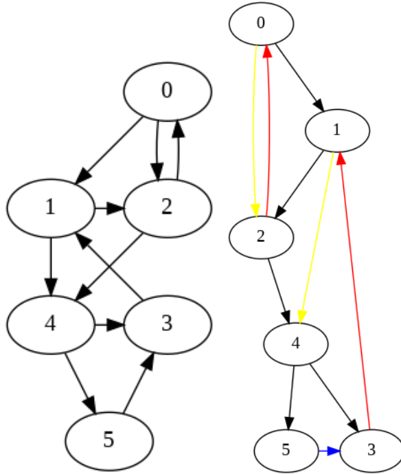
Figure 11.11: Classification of Edges: black marks tree edge, red marks back edge, yellow marks forward edge, and blue marks cross edge.
