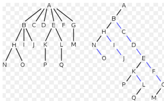
Figure 4.10: A 6-ary Tree Vs a binary tree.
