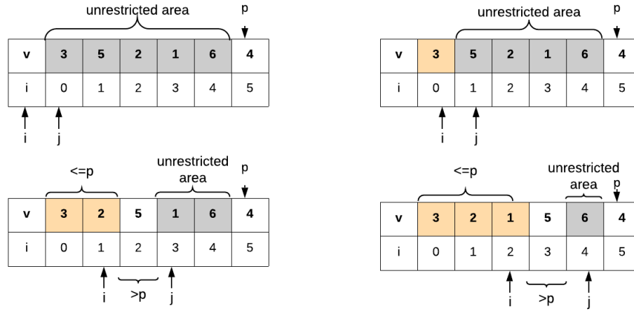
Figure 15.5: Lomuto's Partition. Yellow, white, and gray marks as region (1), (2) and (3), respectively.
