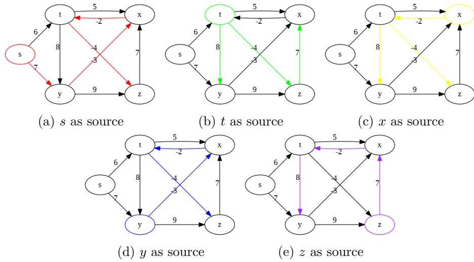
Figure 20.23: All shortest-path trees starting from each vertex.
