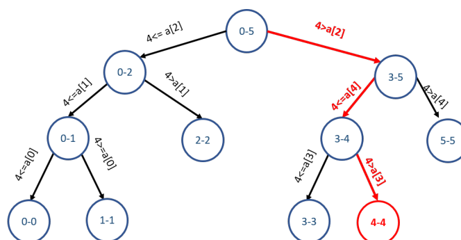
Figure 2.5: Binary Search on an implicit Tree Structure
