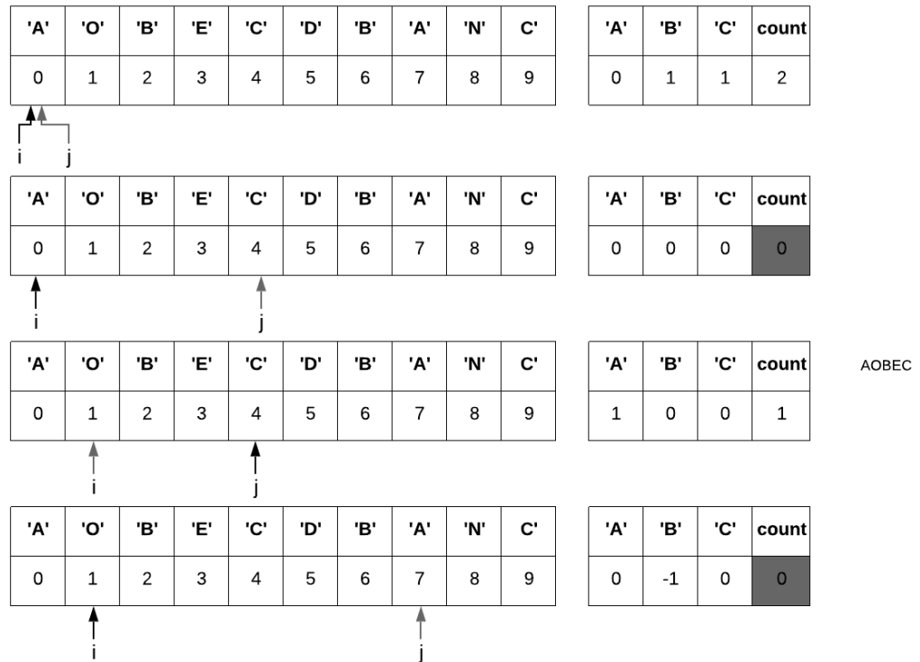
Figure 19.3: The partial process of applying two pointers. The grey shaded arrow indicates the pointer that is on move.
