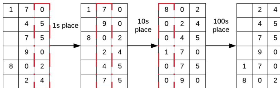
Figure 15.9: Radix Sort: LSD sorting integers in iteration
