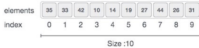
Figure 4.1: Array Representation
