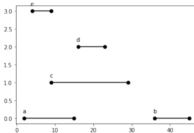
Figure 17.2: All intervals
