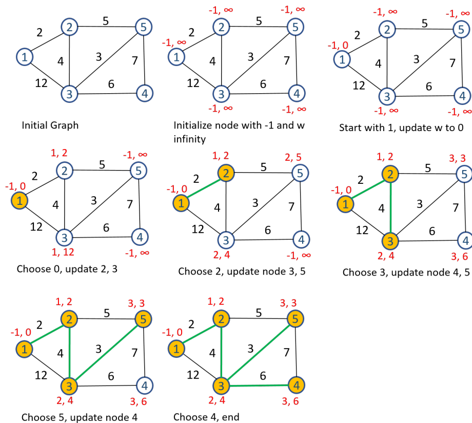
Figure 20.11: Prim's Algorithm
