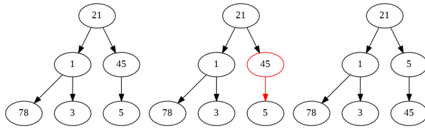
Figure 9.7: Heapify: The last parent node 45.
