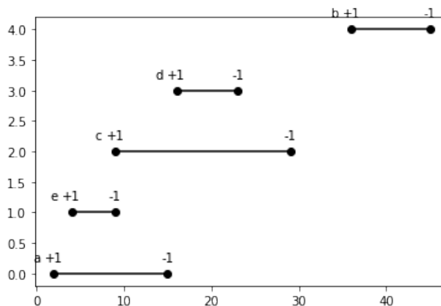
Figure 17.3: All intervals sorted by start and end time.
