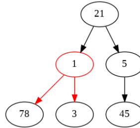
Figure 9.8: Heapify: On node 1
