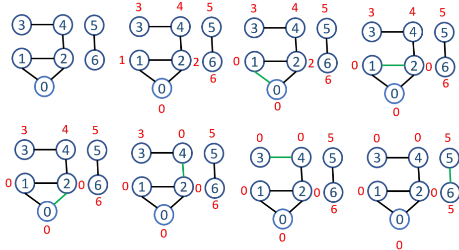
Figure 21.3: A disjoint forest
