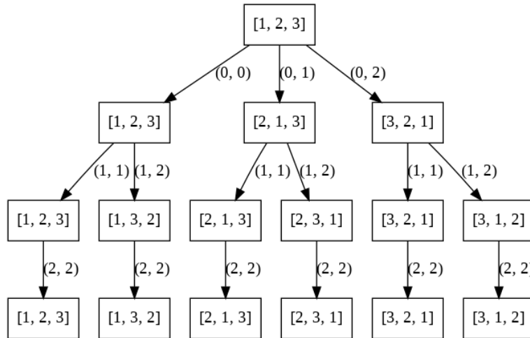
Figure 12.3: The search tree of permutation by swapping. The indexes of items to be swapped are represented as a two element tuple.
