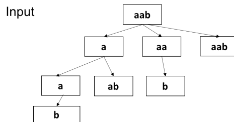
Figure 16.3: State Transfer for the panlindrom splitting
