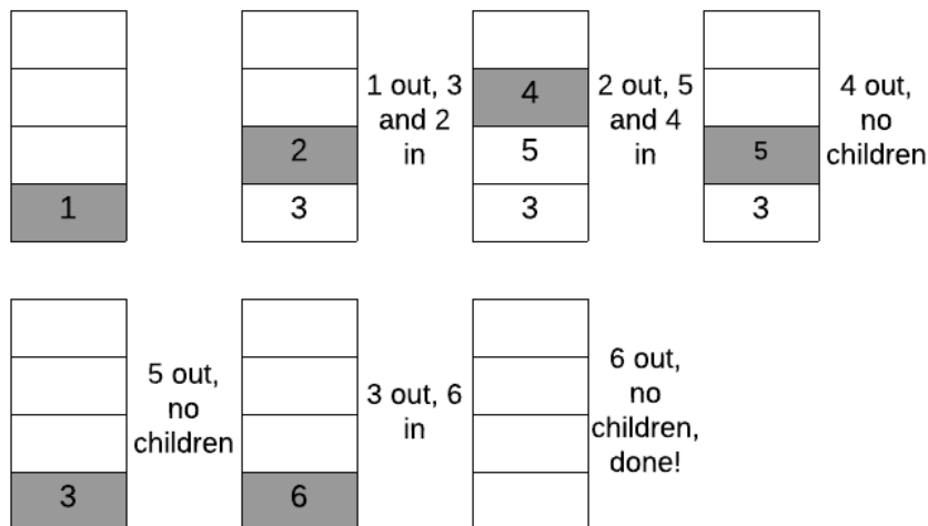
Figure 11.15: The process of iterative preorder tree traversal.
