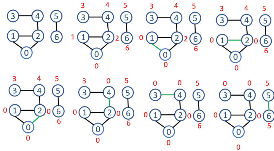
Figure 21.2: The connected components using disjoint set.
