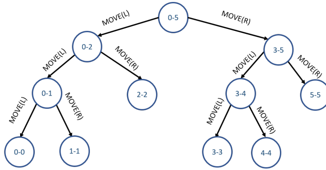
Figure 2.3: State Transfer Process on the tree
