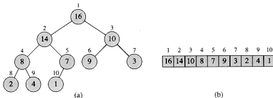
Figure 9.4: Max-heap be visualized with binary tree structure on the left, and be implemented with Array on the right.
