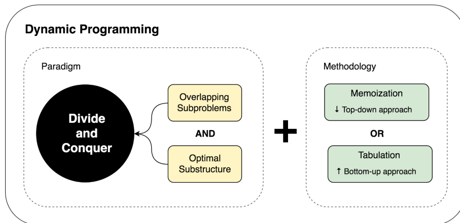
Figure 16.1: Dynamic Programming Chapter Recap
