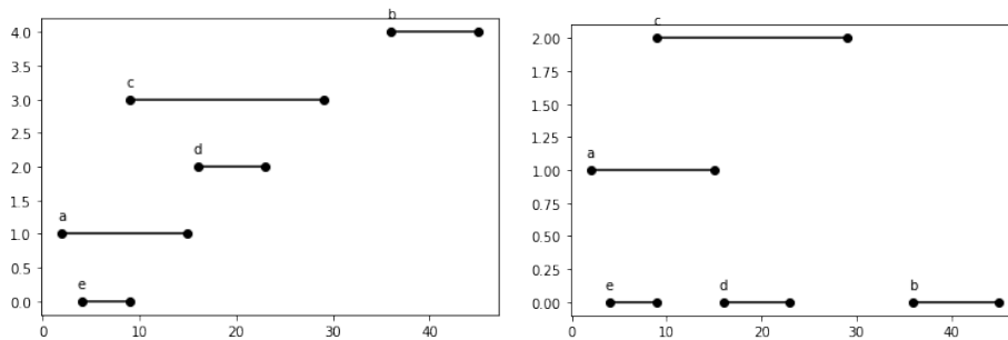
Figure 17.4: Left: sort by start time, Right: sort by finish time.
