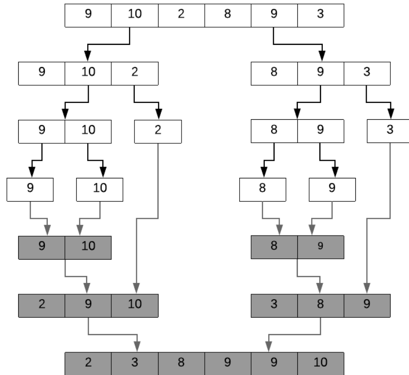
Figure 13.2: Merge Sort with non-overlapping subproblems where subproblems form a tree
