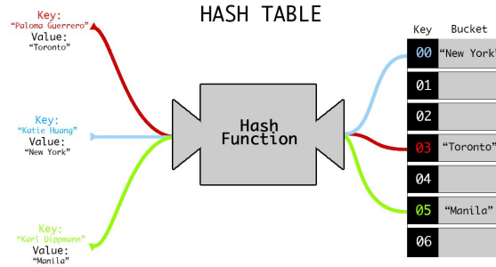
Figure 4.5: Example of Hashing Table, replace key as index
