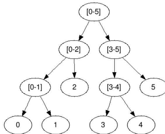
Figure 14.9: A Segment Tree
