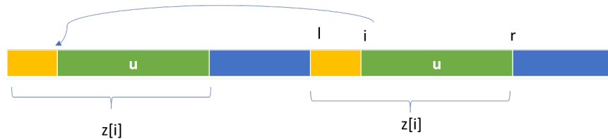
Figure 22.5: Z function property
