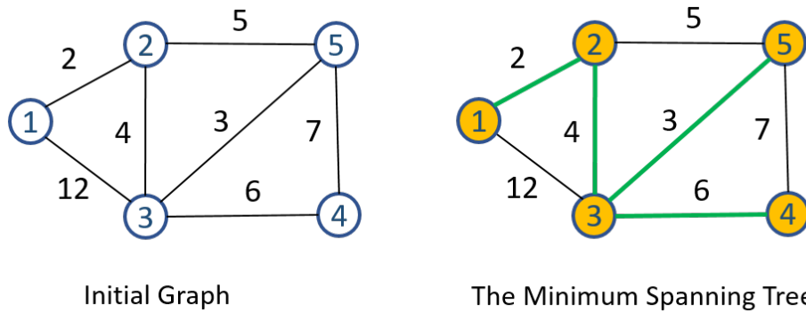
Figure 20.7: Example of minimum spanning tree in undirected graph, the green edges are edges of the tree, and the yellow filled vertices are vertices of MST (change this to a graph with multiple spanning tree, and highlight the one with the minimum ones).
