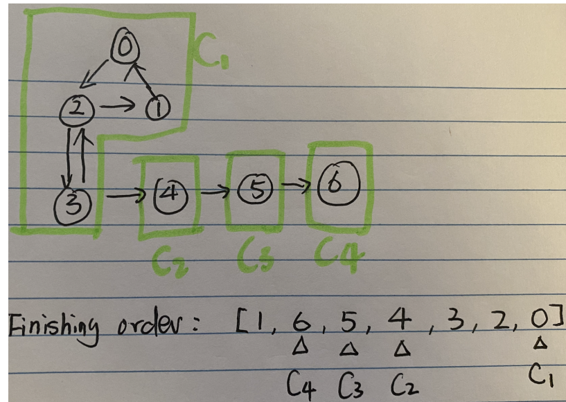
Figure 20.6: A graph with four SCCs.
