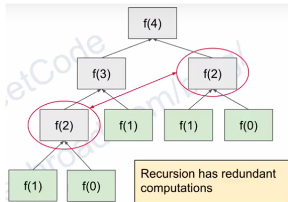
Figure 13.3: Fibonacci number with overlapping subproblems where subproblems form a graph.
