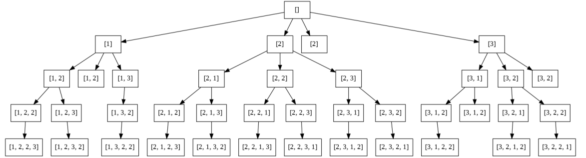
Figure 12.4: The search tree of permutation with repetition
