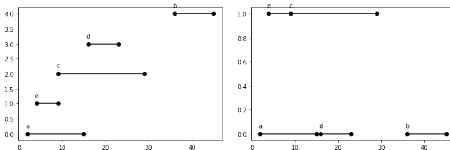
Figure 17.5: Left: sort by start time, Right: sort by finish time.
