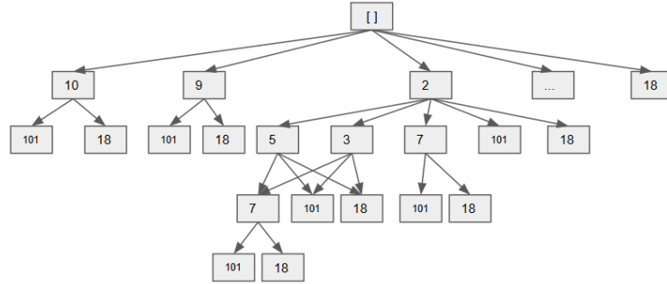
Figure 18.1: Graph Model for LIS, each path represents a possible solution.
