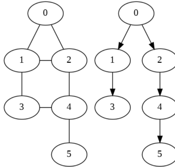
Figure 11.9: Breath-first Graph Search Tree.
