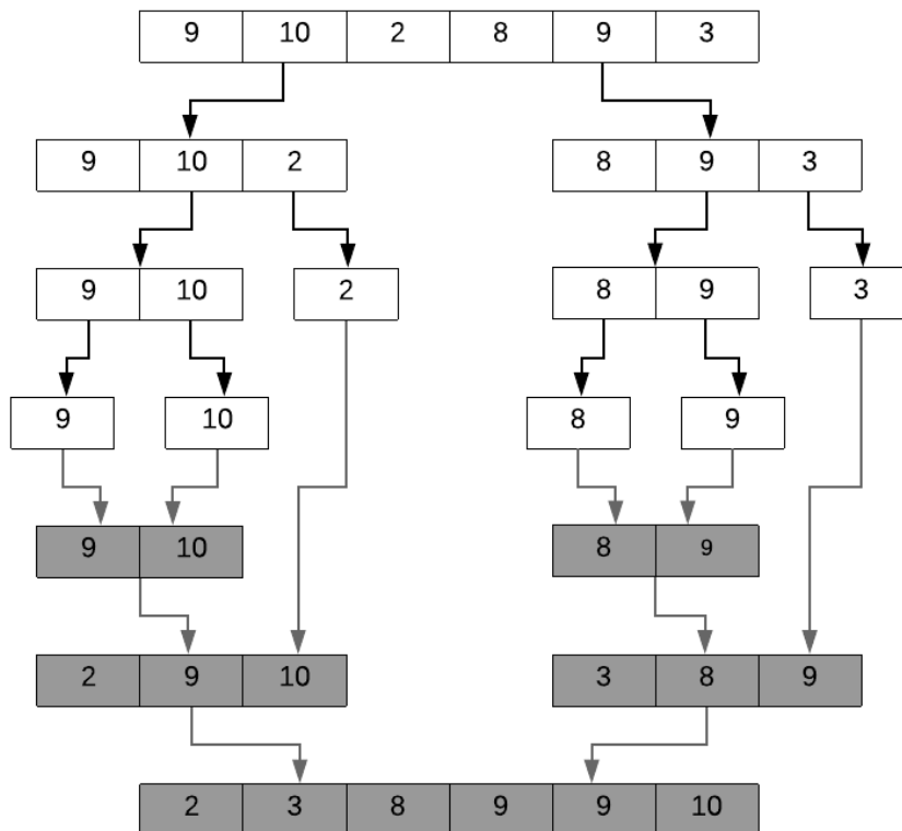
Figure 15.4: Merge Sort: The dividing process is marked with dark arrows and the merging process is with gray arrows with the merge list marked in gray color too.
