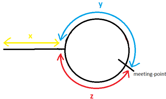
Figure 19.6: Floyd's Cycle finding Algorithm
