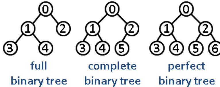
Figure 4.11: Example of different types of binary trees
