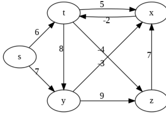
Figure 20.12: A weighted and directed graph.
