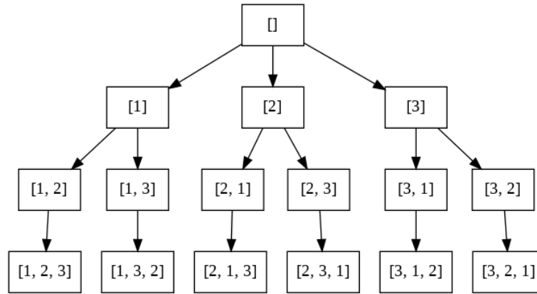
Figure 12.2: The search tree of permutation
