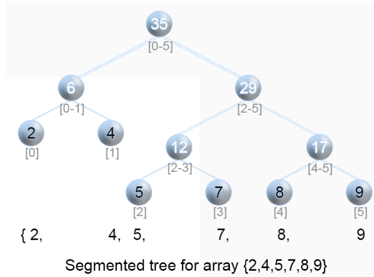
Figure 27.3: Illustration of Segment Tree.
