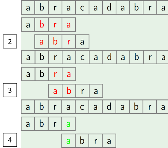
Figure 22.2: The Skipping Rule
