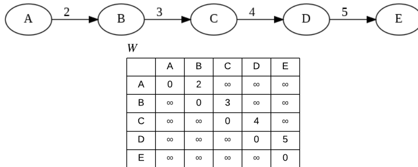
Figure 20.14: The simple graph and its adjacency matrix representation (changing it to lower letter)
