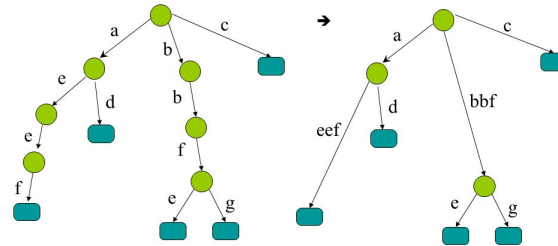
Figure 27.4: Trie VS Compact Trie
