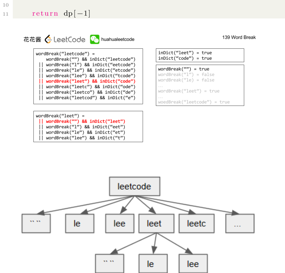
Figure 29.2: Word Break with DFS. For the tree, each arrow means check the word = parent-child and then recursively check the result of child.
