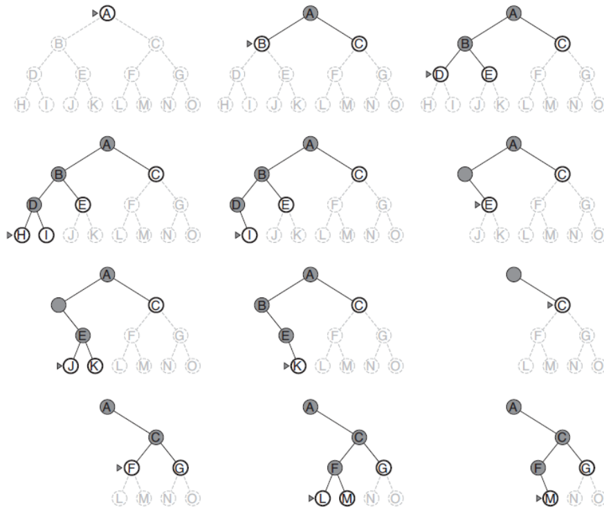
Figure 11.4: Depth-first search on a simple search tree. The unexplored region is shown in light gray. Explored nodes with no descendants in the frontier are removed from memory as node L disappears. Dark gray marks nodes that is being explored but not finished.
