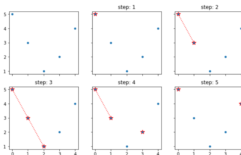
Figure 21.1: The process of decreasing monotone stack
