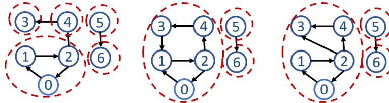
Figure 20.5: The strongly connected components in directed graph, each dashed red circle marks a strongly connected component.
