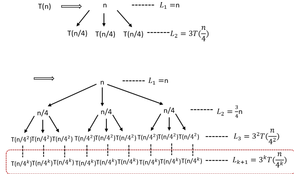
Figure 10.3: The process to construct a recursive tree for T(n) = 3T(\lfloor n/4 \rfloor) + O(n) . There are totally k+1 levels. Use a better figure.
