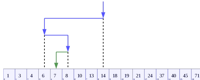
Figure 14.1: Example of Binary Search
