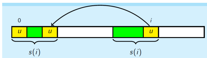
Figure 22.4: Proof of Lemma
