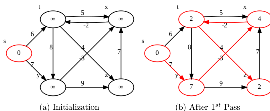
Figure 20.20: The execution of Bellman-Ford's Algorithm with ordering [s, t, y, z, x] .
