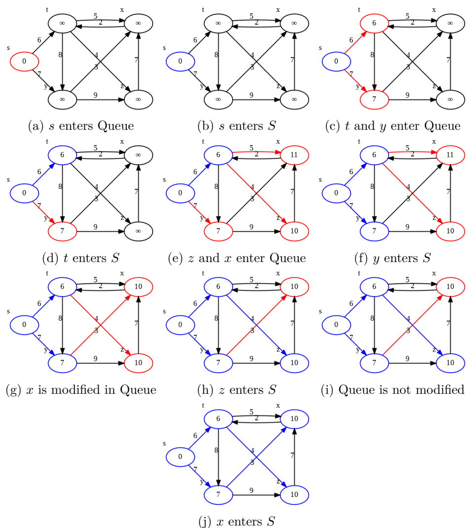
Figure 20.22: The execution of Dijkstra's Algorithm on non-negative weighted graph. Red circled vertices represent the priority queue, and blue circled vertices represent the set S . Eventually, the blue colored edges represent the shortest-paths tree.
