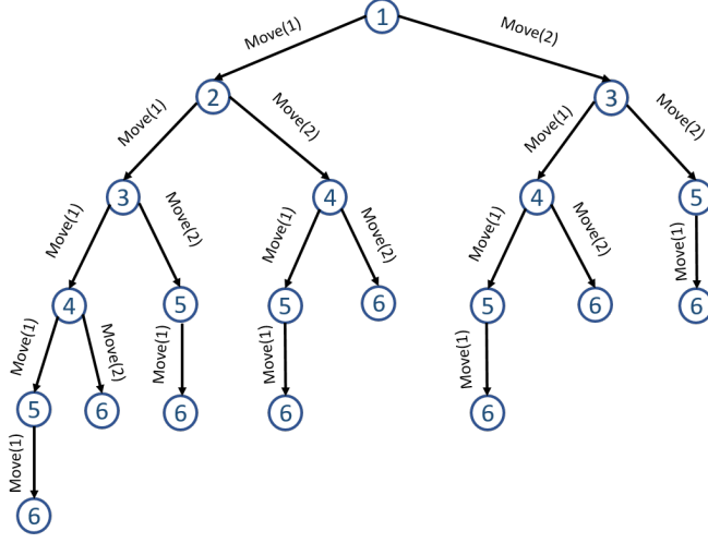
Figure 2.1: The State Space Graph. This may appears as a tree, but we can redraw it as a graph.
