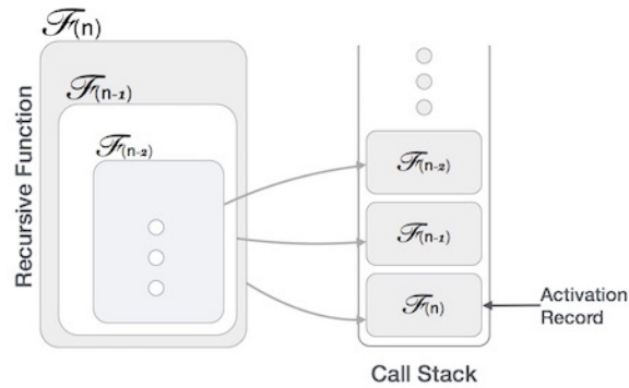
Figure 7.2: Call stack of recursion function
