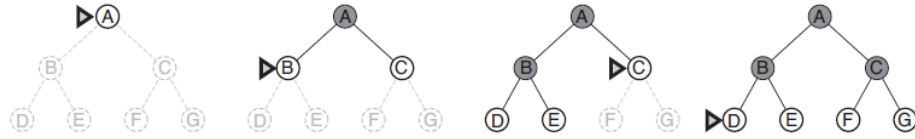
Figure 11.3: Breadth-first search on a simple search tree. At each stage, the node to be expanded next is indicated by a marker.
