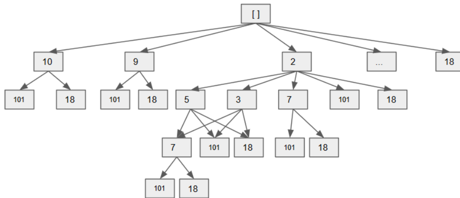
Figure 2.7: State Transfer Tree Structure for LIS, each path represents a possible solution. Each arrow represents an move: find an element in the following elements that's larger than the current node.
