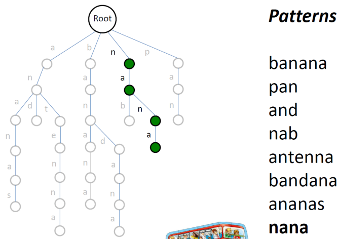
Figure 22.7: Building a Trie from Patterns
