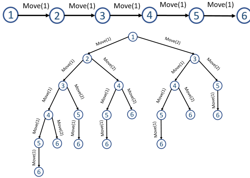
Figure 2.6: The State Spaces Graph
