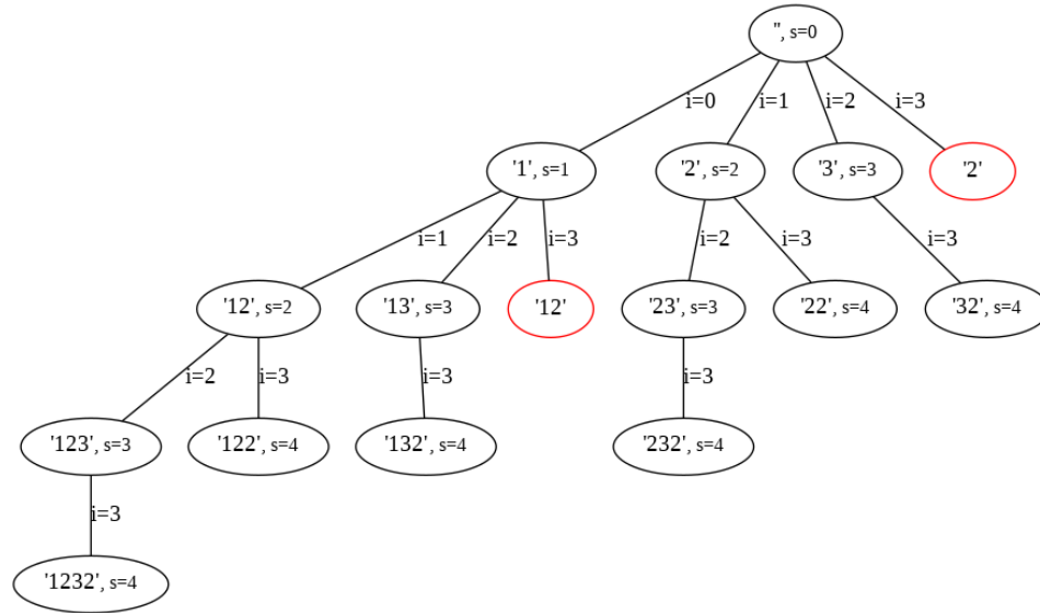
Figure 12.7: The Search Tree of subsequences. The red circled nodes are redundant nodes. Each node has a variable s to indicate the starting index of candidates to add to current subsequence. i indicate the candidate to add to the current node.
