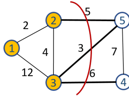
Figure 20.9: A cut denoted with red curve partition V into \{1,2,3\} and \{4,5\} .
