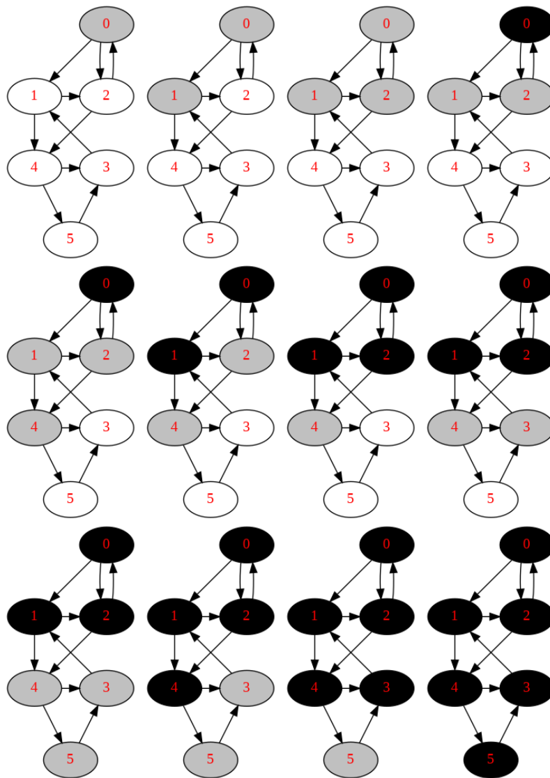
Figure 11.12: The process of Breath-first Graph Search. The black arrows denotes the the relation of u and its not visited neighbors v . And the red arrow marks the backtrack edge.
