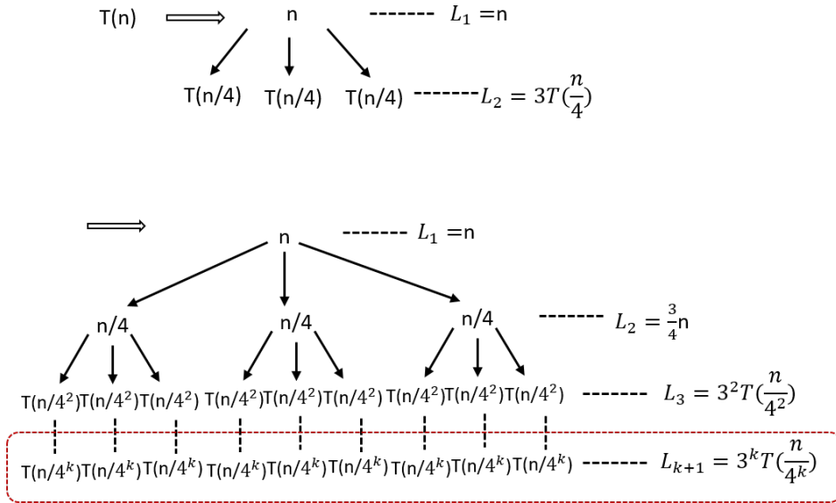
Figure 6.1: The process to construct a recursive tree for T(n) = 3T(\lfloor n/4 \rfloor) + O(n) . There are totally k+1 levels. Use a better figure.
