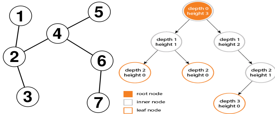
Figure 4.9: Example of Trees. Left: Free Tree, Right: Rooted Tree with height and depth denoted
